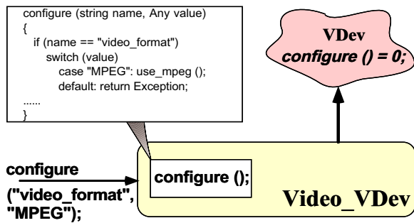
Figure 6: Virtual Device
